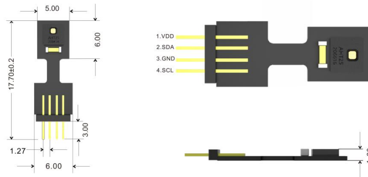
Figure 12. AHT25 sensor encapsulation (unit: mm unmarked tolerance: \pm 0.1\text{mm} )
